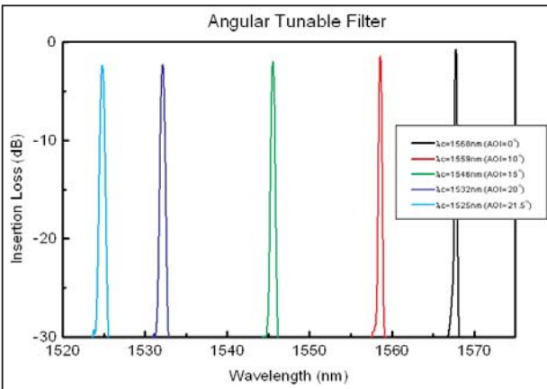
Fig 4: Tuning Curve for Angular Tunable Filter
